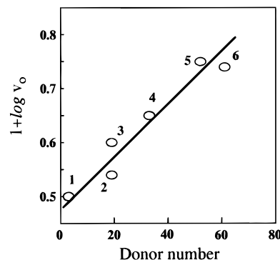
FIGURE 3. Correlation between the initial rate of CH_3CHO ( H_2 ) formation from species 2 and the donor number of nucleophilic compounds ( 1 , CH_3NO_2 ; 2 , (C_2H_5)_2O ; 3 , THF; 4 , C_5H_5N ; 5 , C_5H_{11}N ; 6 , (C_2H_5)_3N ).
